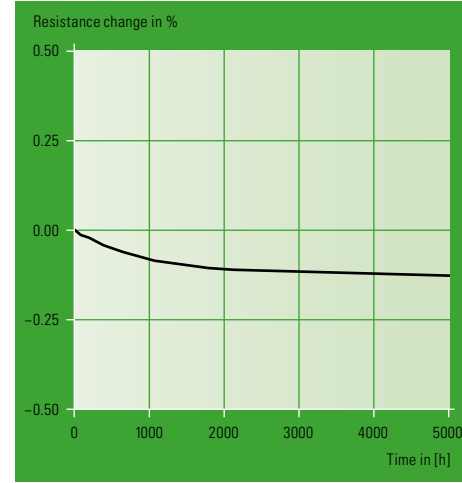
Long-term stability: MANGANIN®
